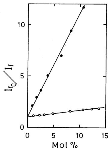
Fig. 3. Effect of addition of polar solvents on the intensity of fluorescent light of 3b in benzene (ordinate: relative fluorescence intensities; abscissa: mol% of polar solvents in benzene).
